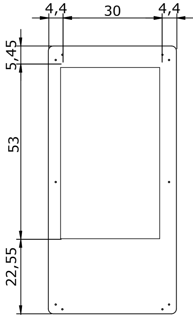
FRONTE plex sp:5mm
