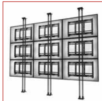
3x3 LANDSCAPE VIDEO WALL Shown in Modular Series Dual Pole Floor-to-Ceiling configuration (SmartMount® Full Service Video Wall Mount with Quick Release, DS-VW765-LQR, required)
